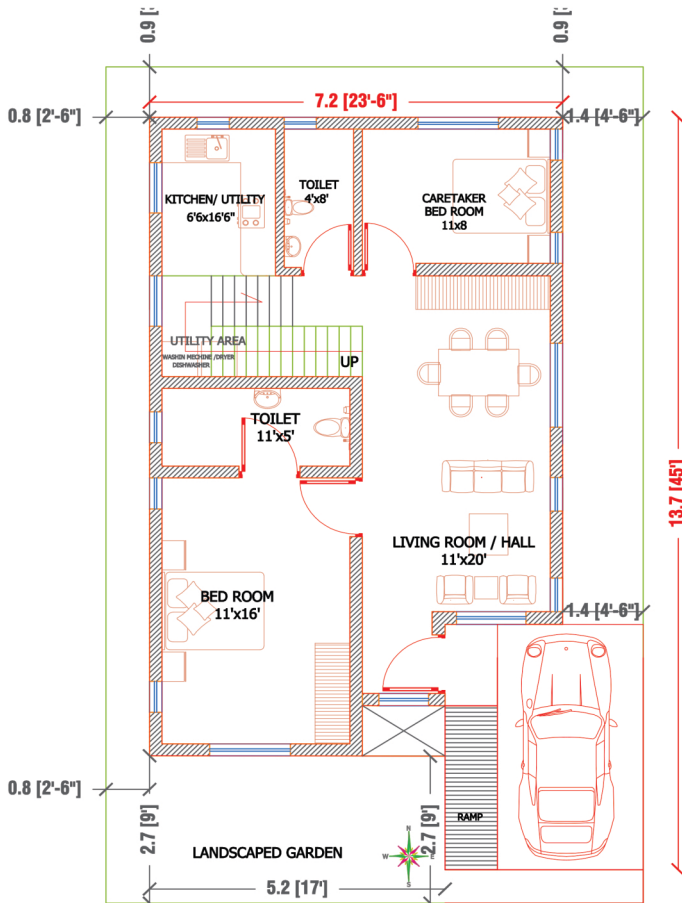
SOUTH FACING OPTION 4 GROUND FLOOR PLAN
